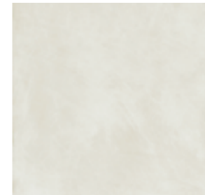
a Chalk
