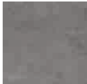
c Iron
